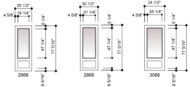
Hinged Patio Door - Outswing
